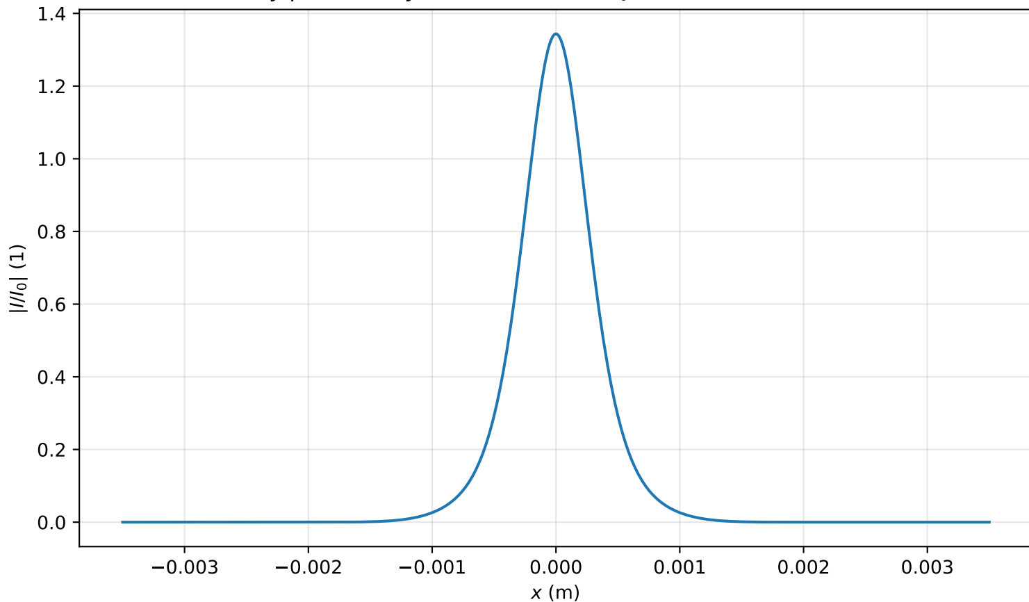
Intensity profile I(x, y = 0, z = 1.274m)/I_0 , P_{in}=0.8P_{cr} , artificial time
